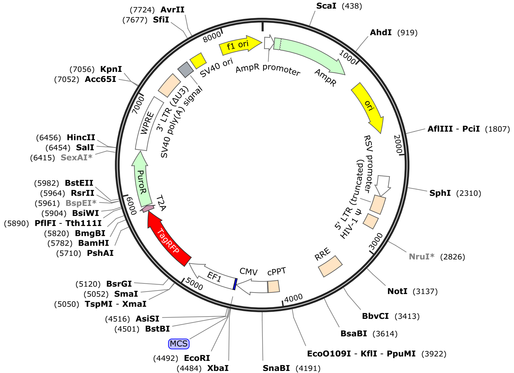
Collecta-pRCDCMERP-CMV-MCS-EF1-TagRFP-2A-Puro
