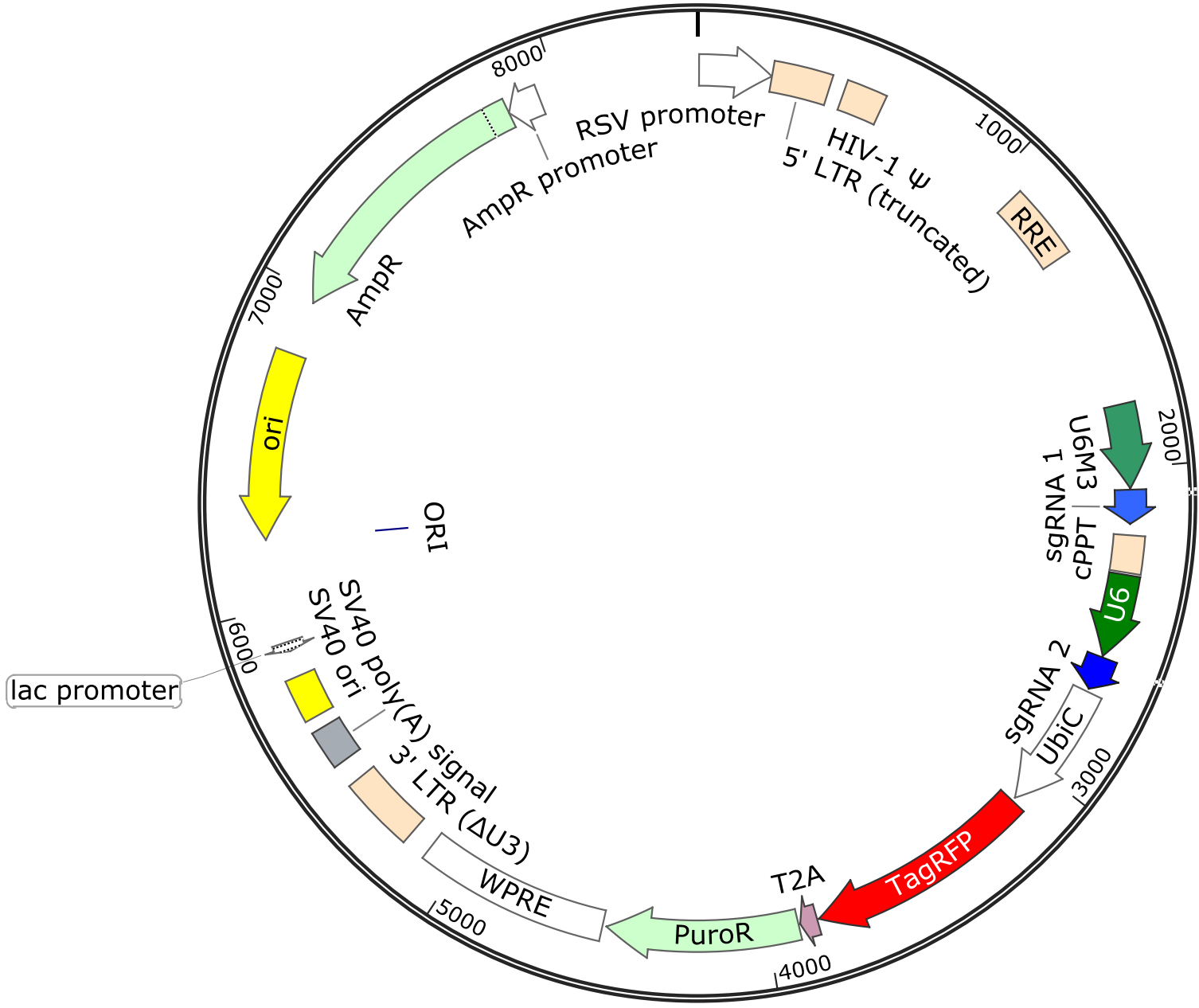
Collecta-pRDSG16-U6M3-sg1-U6-sg2-UbiC-TagRFP-2A-Puro 8437 bp
