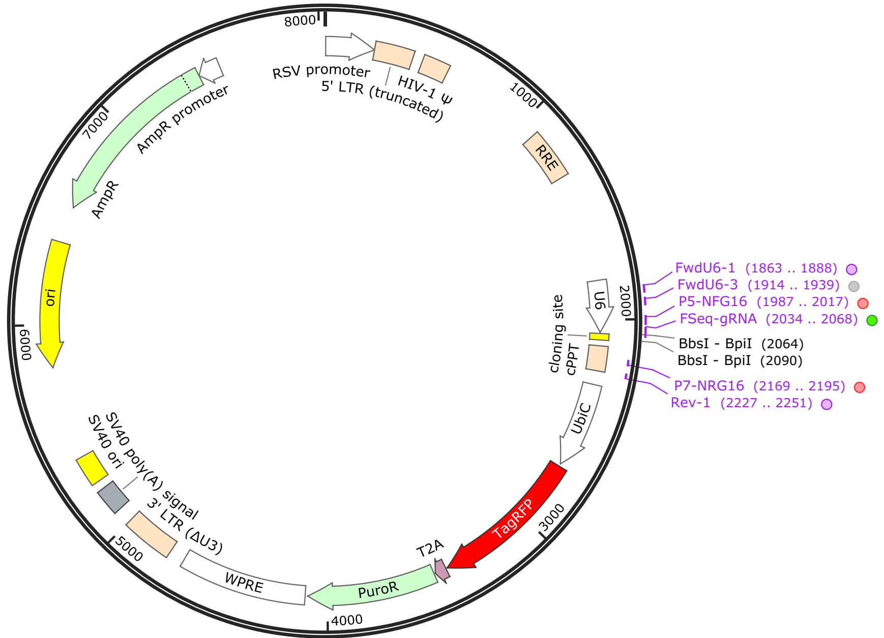
Collecta-pRSG16-U6-sg-HTS6C-UbiC-TagRFP-2A-Puro 8025 bp
