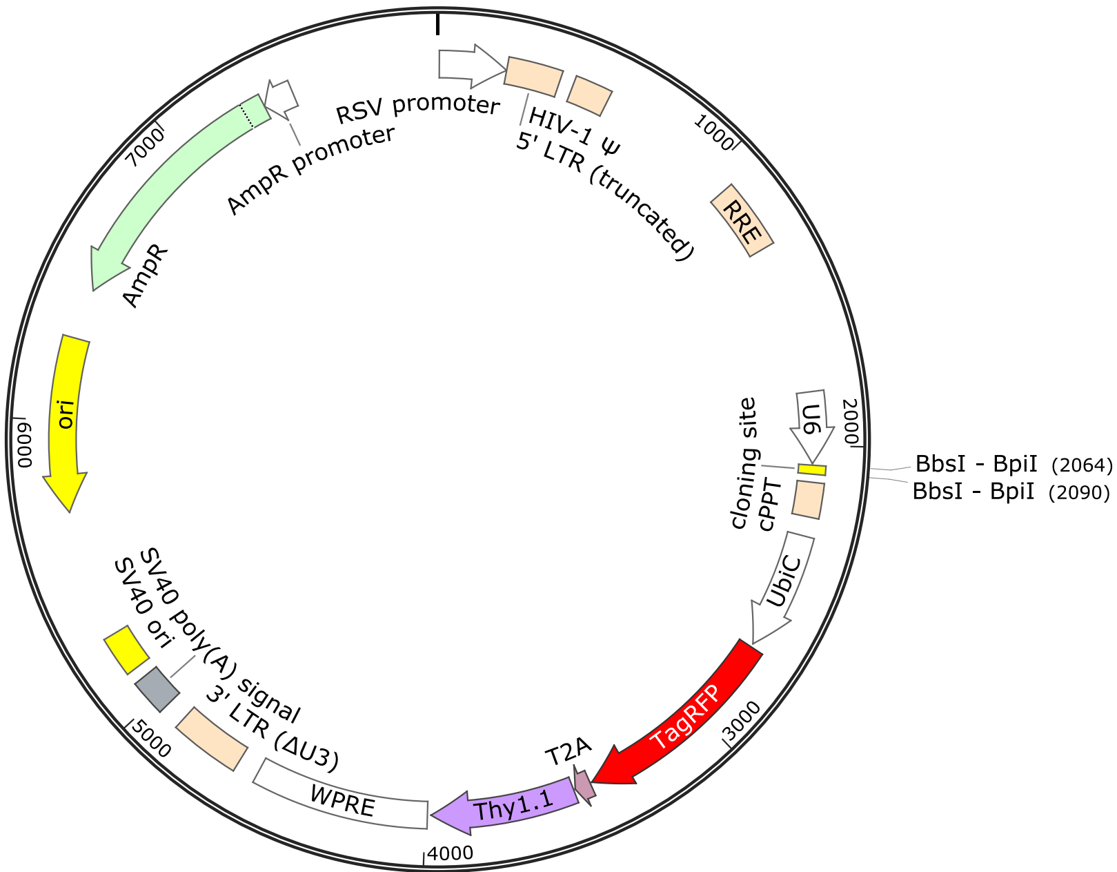
Collecta-pRSG16Thy-U6-sg-HTS6C-UbiC-TagRFP-2A-Thy1.1 7914 bp
