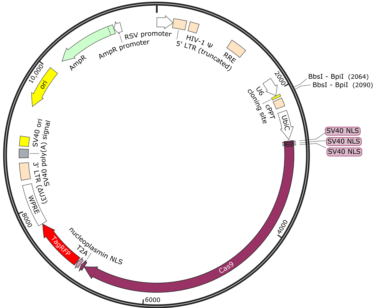
Collecta-pRSGCUR-U6-sg-HTS6C-UbiC-Cas9-2A-TagRFP 11,662 bp
