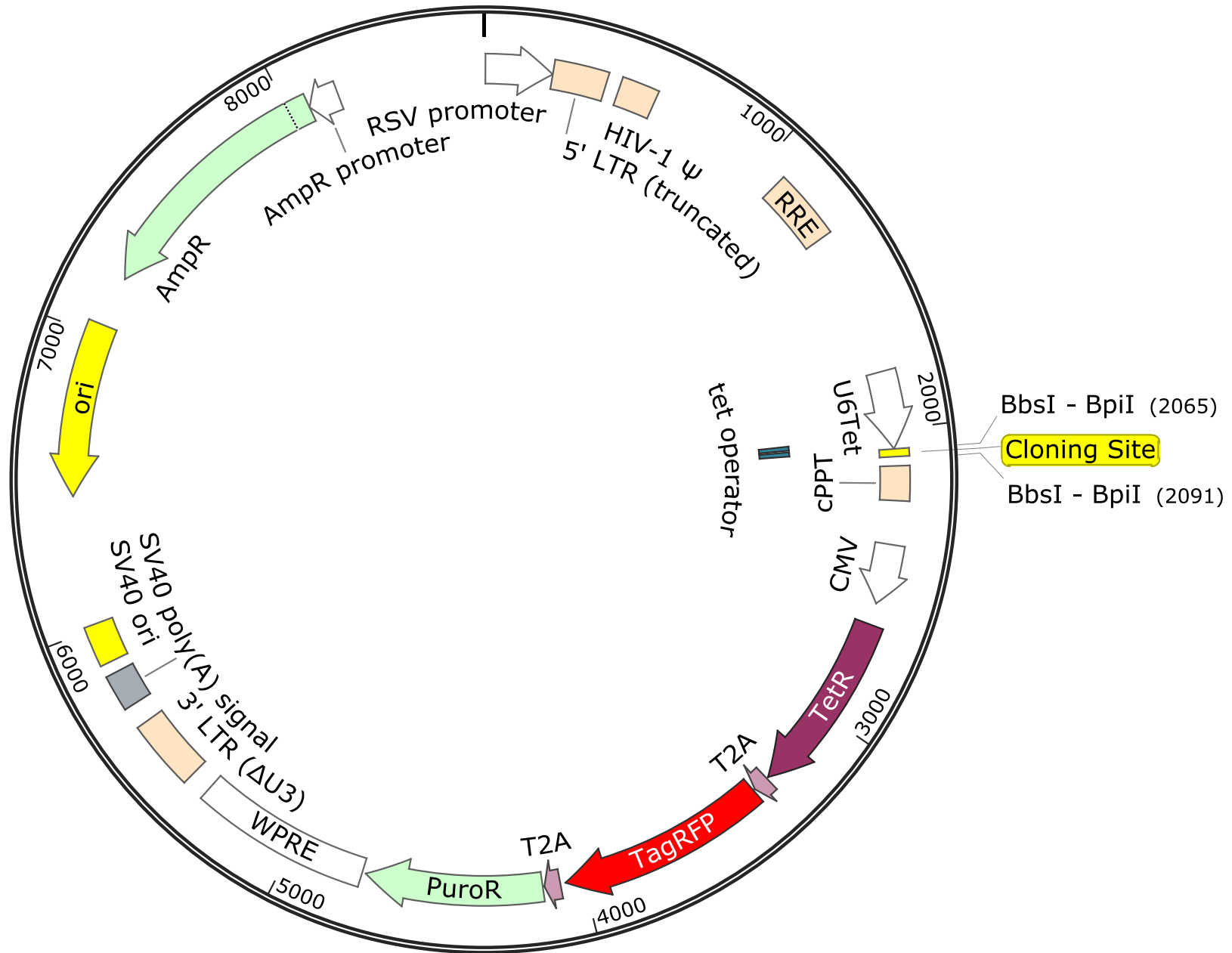
Collecta-pRSGT16-U6Tet-sg-HTS6CTet-CMV-TetRep-2A-TagRFP-2A-Puro
