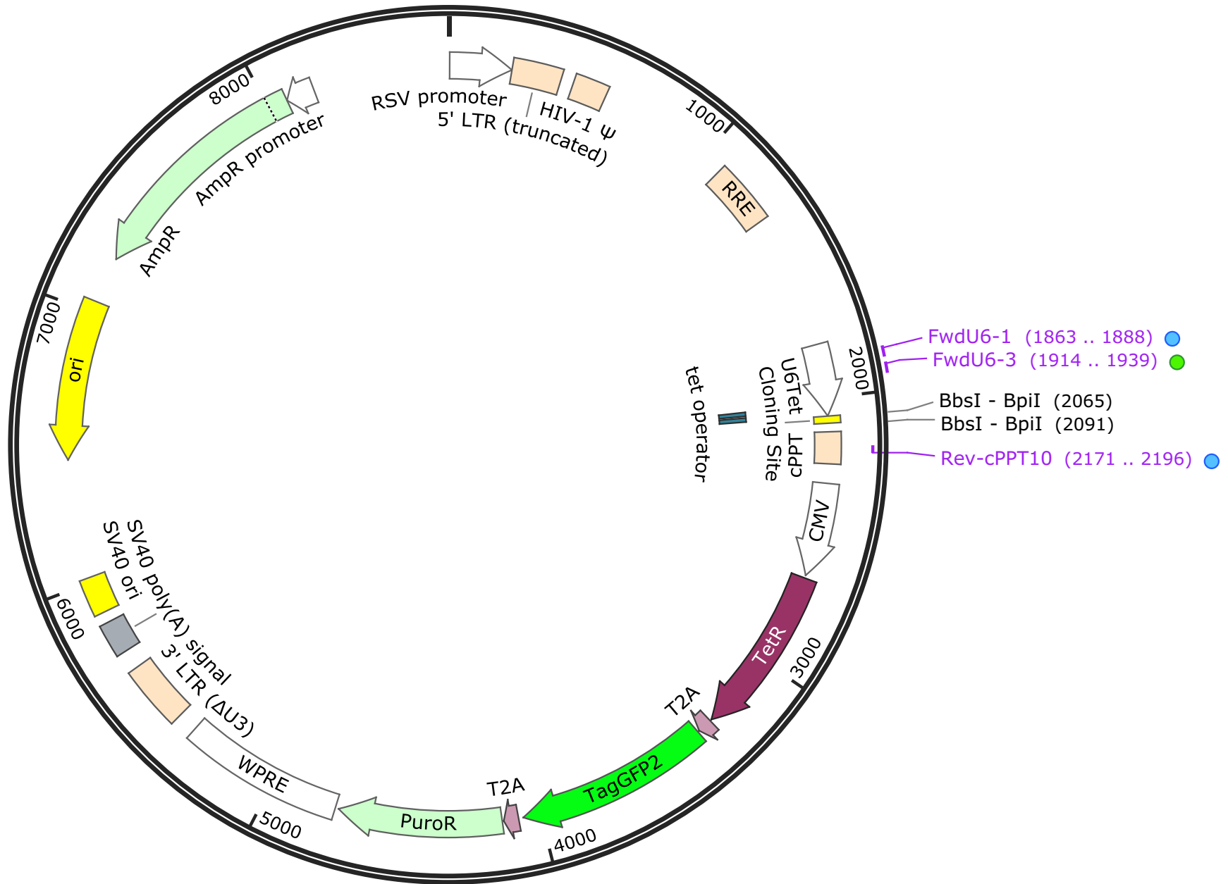
Collecta-pRSGT17-U6Tet-sg-HTS6CTet-CMV-TetRep-2A-TagGFP2-2A-Puro 8676 bp
