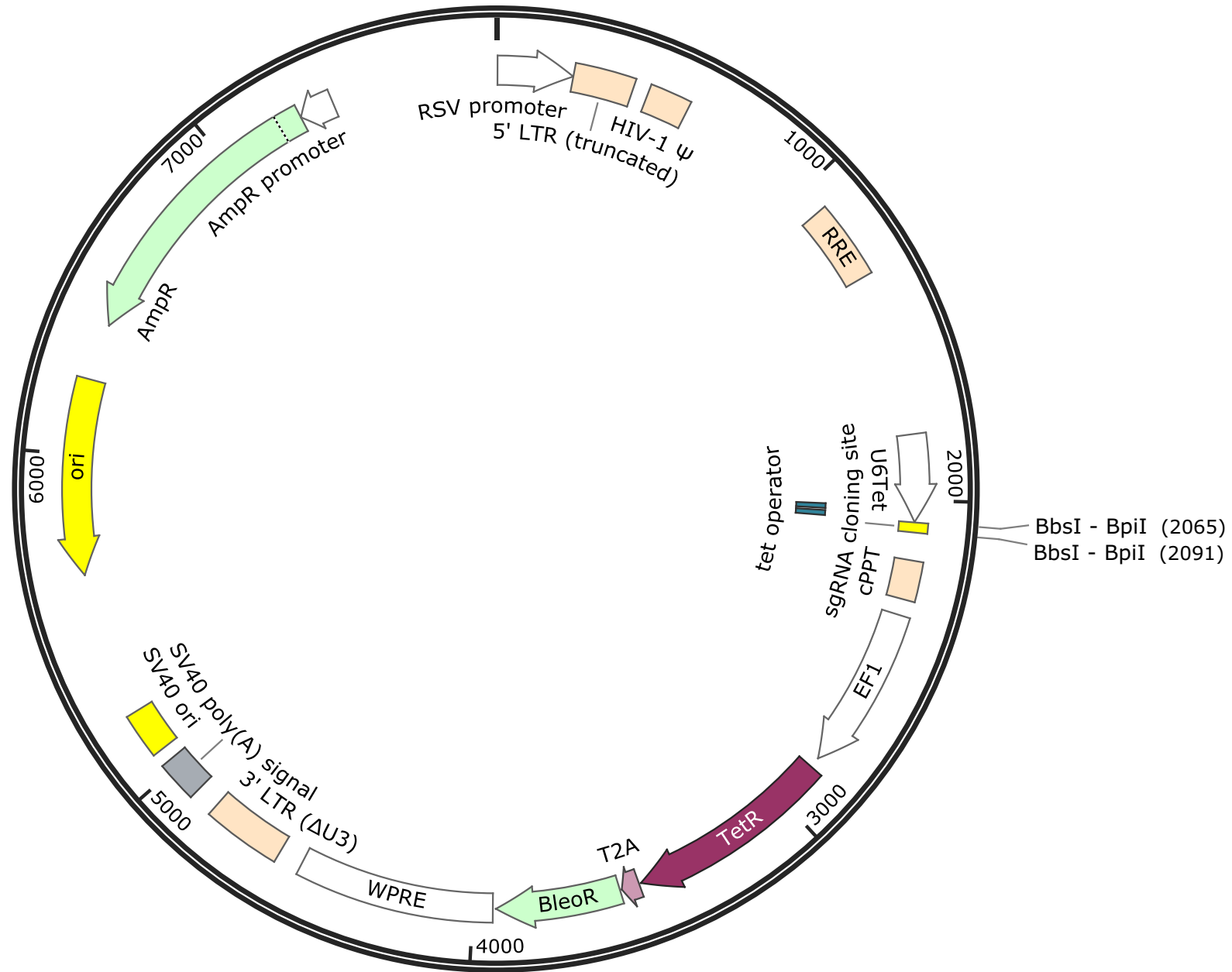
Collecta-pRSGTEbleo-U6Tet-sg-EF1-TetRep-2A-Bleo 7862 bp
