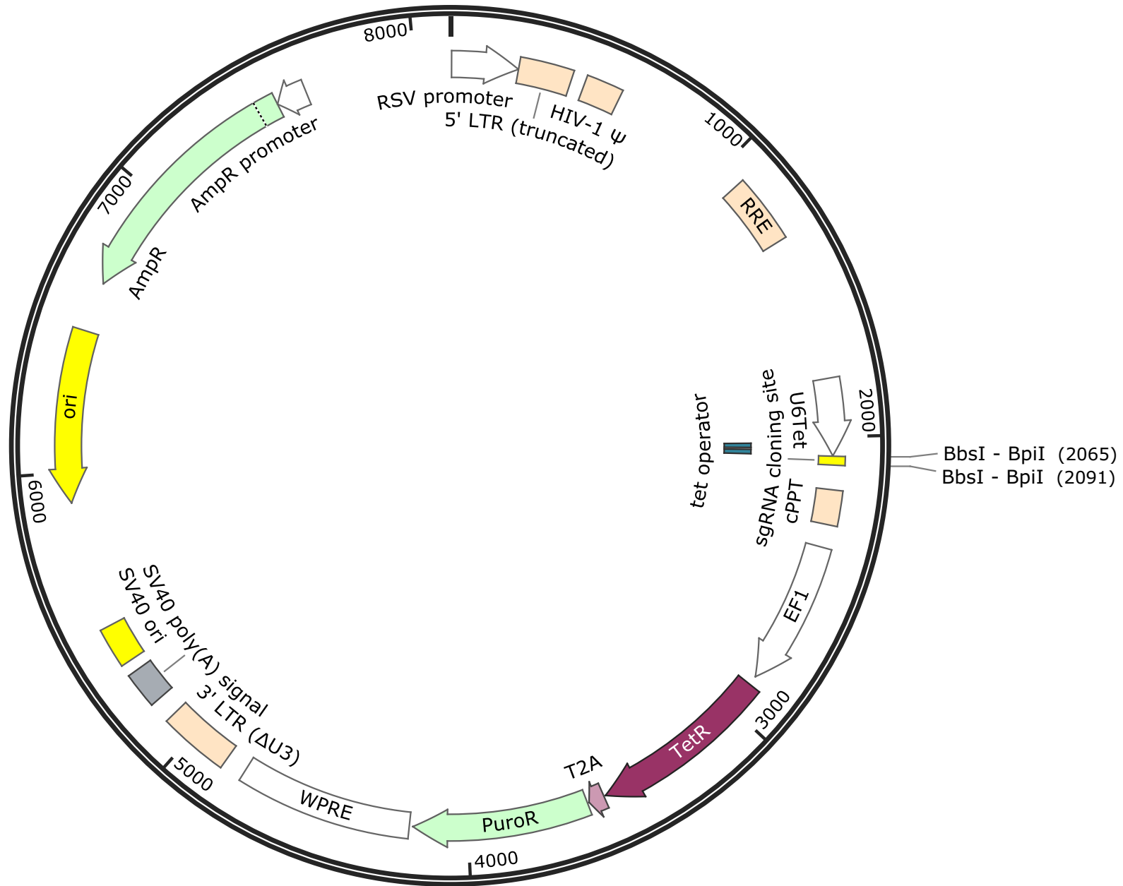
Collecta-pRSGTEP-U6Tet-sg-EF1-TetRep-2A-Puro 8120 bp
