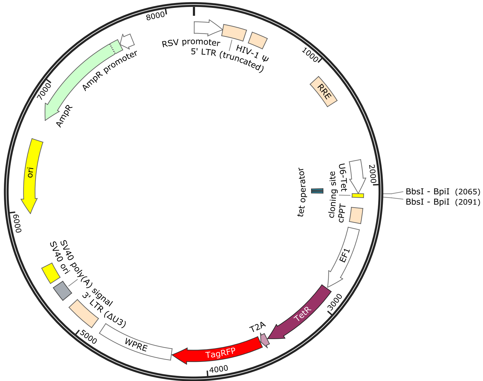
Collecta-pRSGTER-U6Tet-sg-EF1-TetRep-2A-TagRFP 8198 bp
