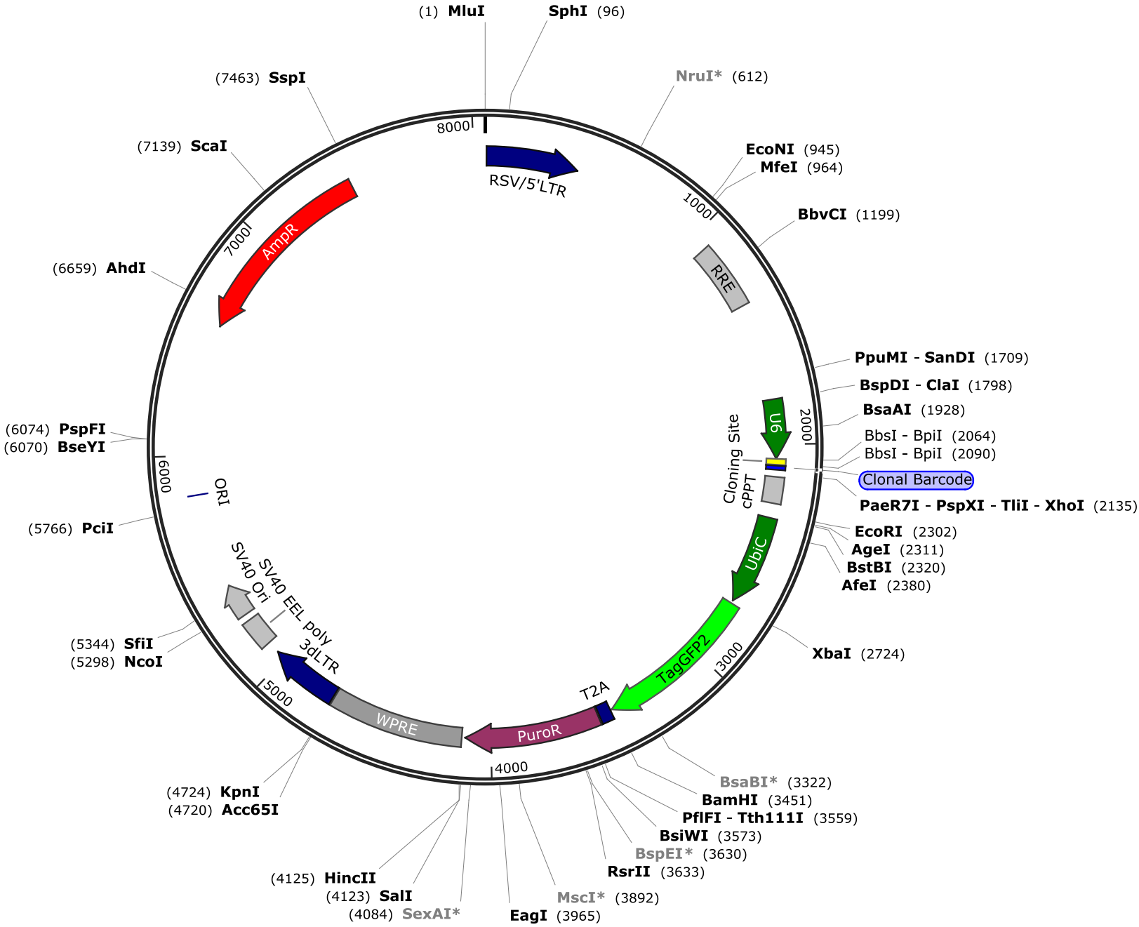
Collecta-pRSI17cb-U6-sh-13kCB18-HTS6cb-UbiC-TagGFP2-2A-Puro 8050 bp
