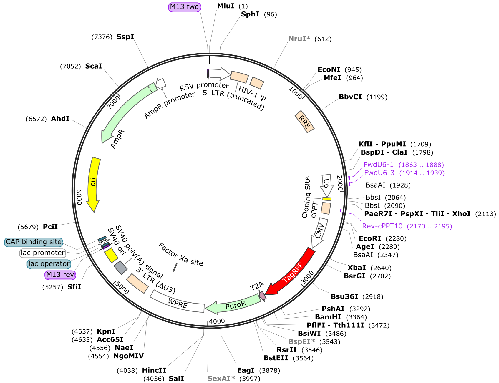
Collecta-pRSI20-U6-sh-HTS6-CMV-TagRFP-2A-Puro
