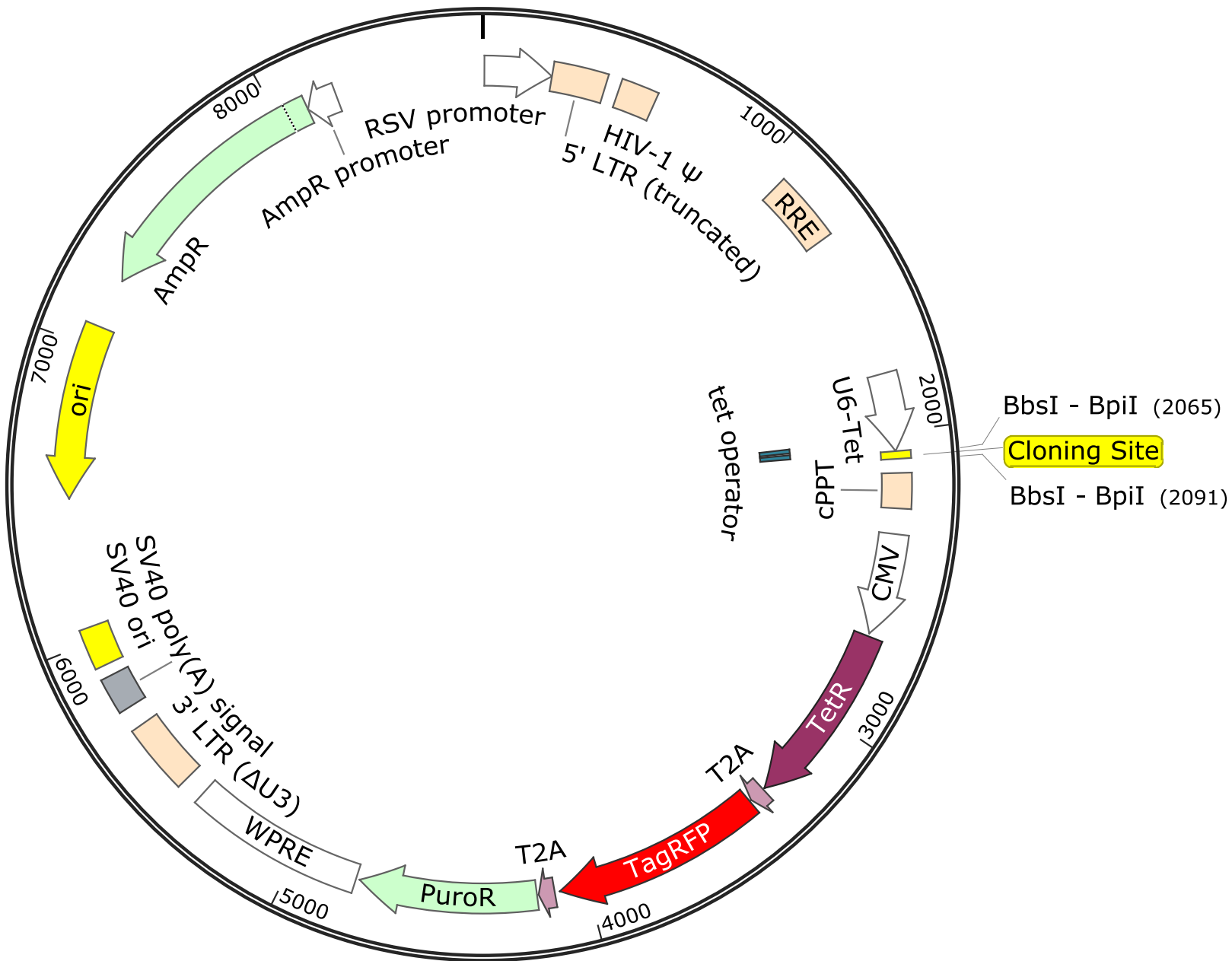
Collecta-pRSIT12-U6Tet-sh-HTS4-CMV-TetRep-2A-TagRFP-2A-Puro 8706 bp
