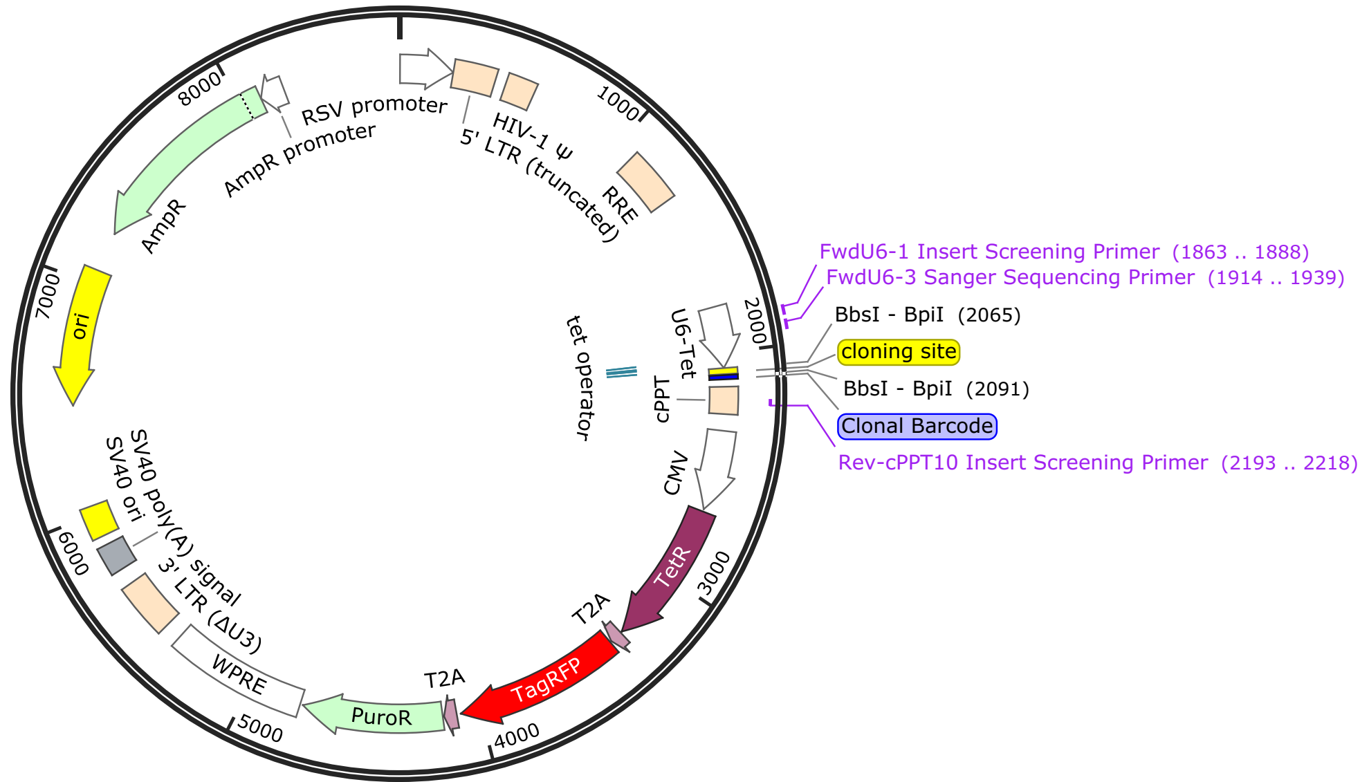
Collecta-pRSIT16cb-U6Tet-sh-13kCB18-HTS6cb-CMV-TetRep-2A-TagRFP-2A-Puro
