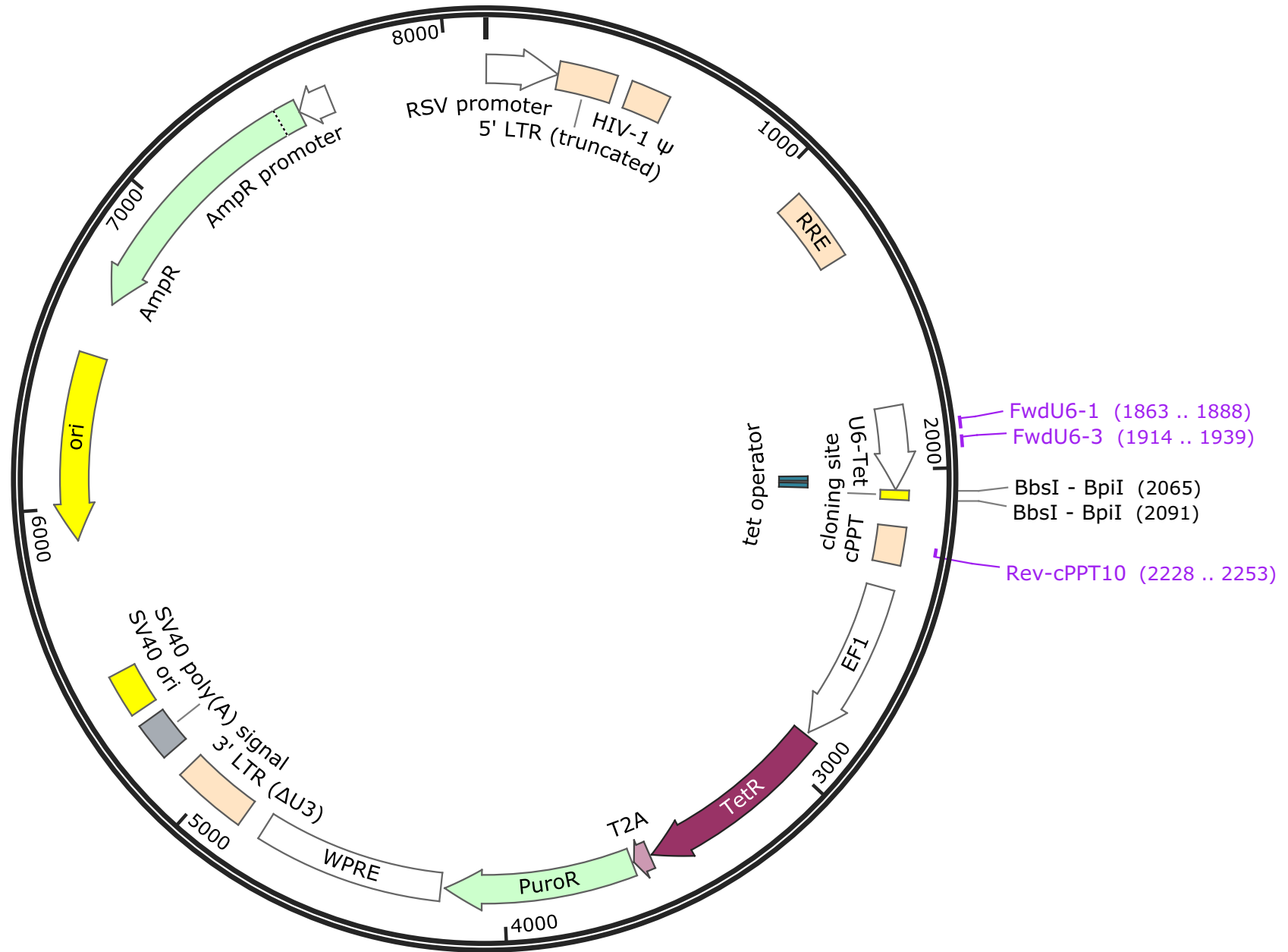
Collecta-pRSITEP-U6Tet-sh-EF1-TetRep-2A-Puro 8120 bp
