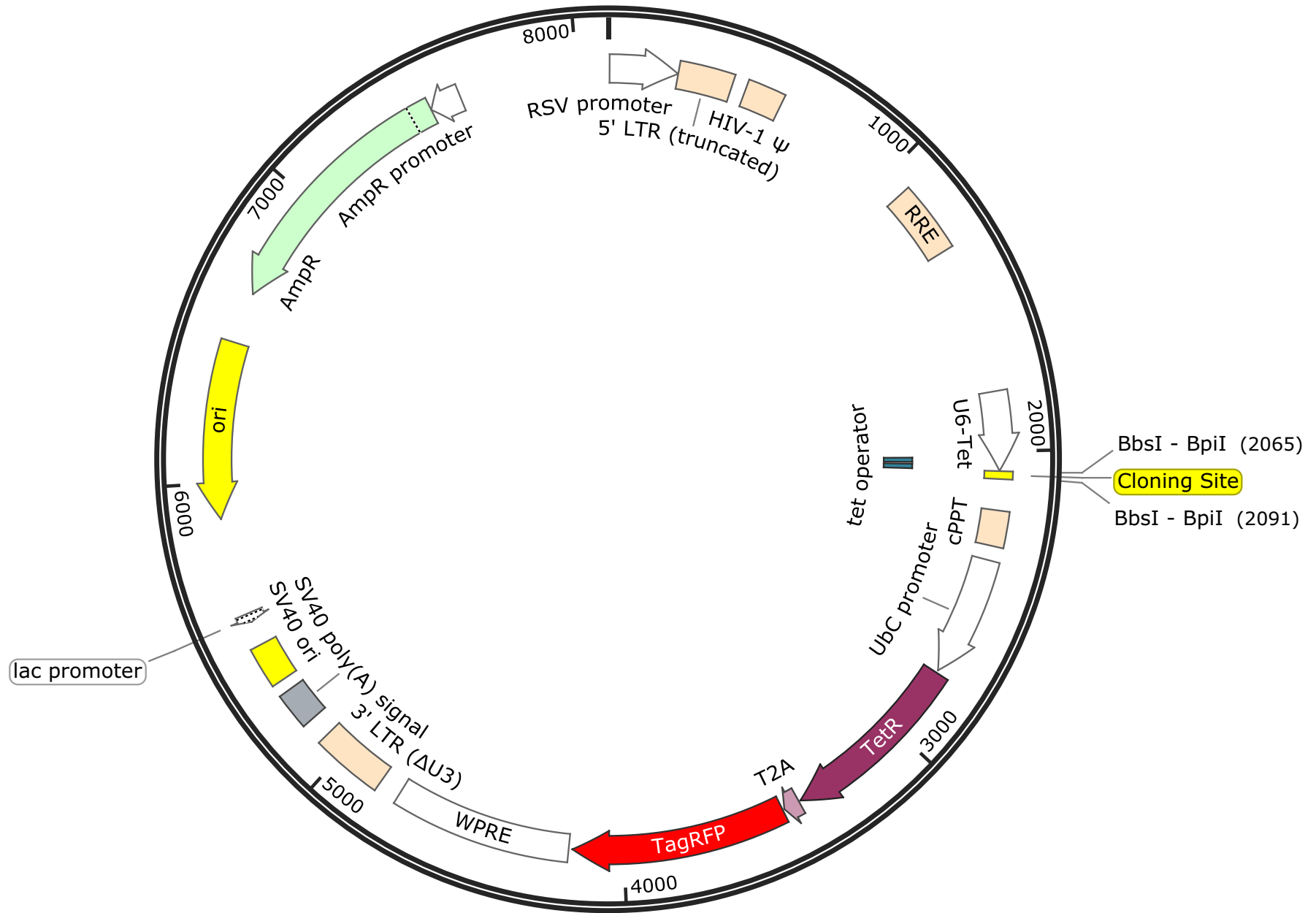
Collecta-pRSITUR-U6Tet-sh-HTS3-UbiC-TetRep-2A-TagRFP 8104 bp
